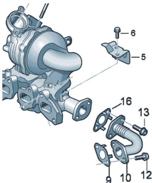
Fig. 2. Diagram of the adapter components required for installation (positions: 5, 6, 9, 10, 12, 13, 16).
